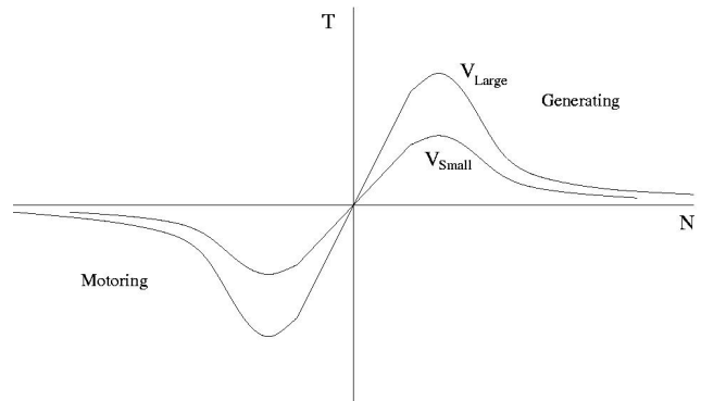
Torque-Speed curve of an asynchronous (induction) machine at different phase voltages.
