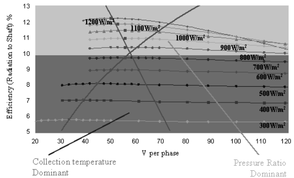
Numerical model variation of net efficiency with infinite bus voltage
