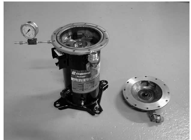
Retrofitted terrestrial refrigeration scroll compressor after capping and flanging.
