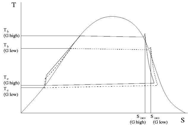
T-S diagrams of possible ORCs under different conditions using retrograde and non-retrograde working fluids.
