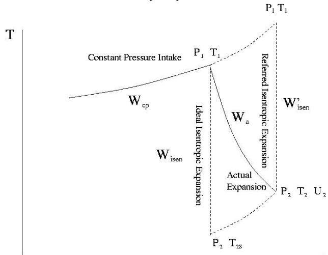
Graphical representation of the extrapolation technique used to obtain isentropic expansion efficiencies
